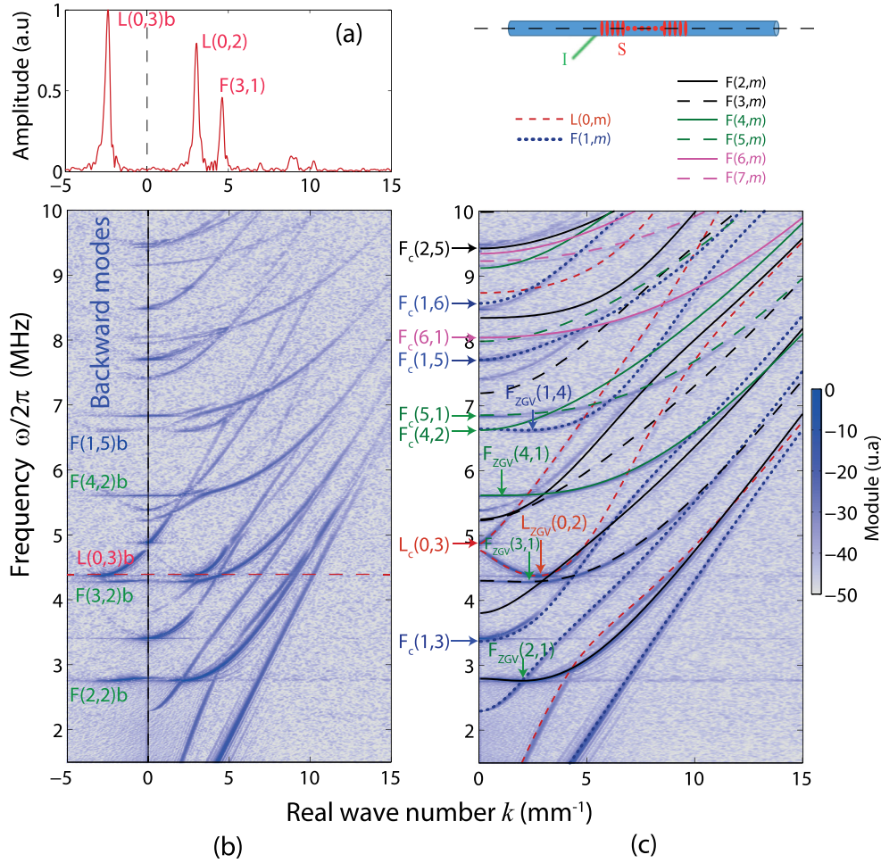
FIG. 5. (Color online) (a) Spatial Fourier transform of the normal displacement at 4.40 MHz illustrating backward propagation with a negative wave number. Each backward mode is coupled to the upper mode of the same family ( n, m + 1 ). To avoid confusion they are indicated by the index b . (b) Experimental dispersion curves obtained for negative and positive wave numbers. (c) Negative dispersion curves \omega(-k) were folded and added to the positive ones. The experimental dispersion curves were fitted with the TI model (the control parameters used are listed in Table I).
