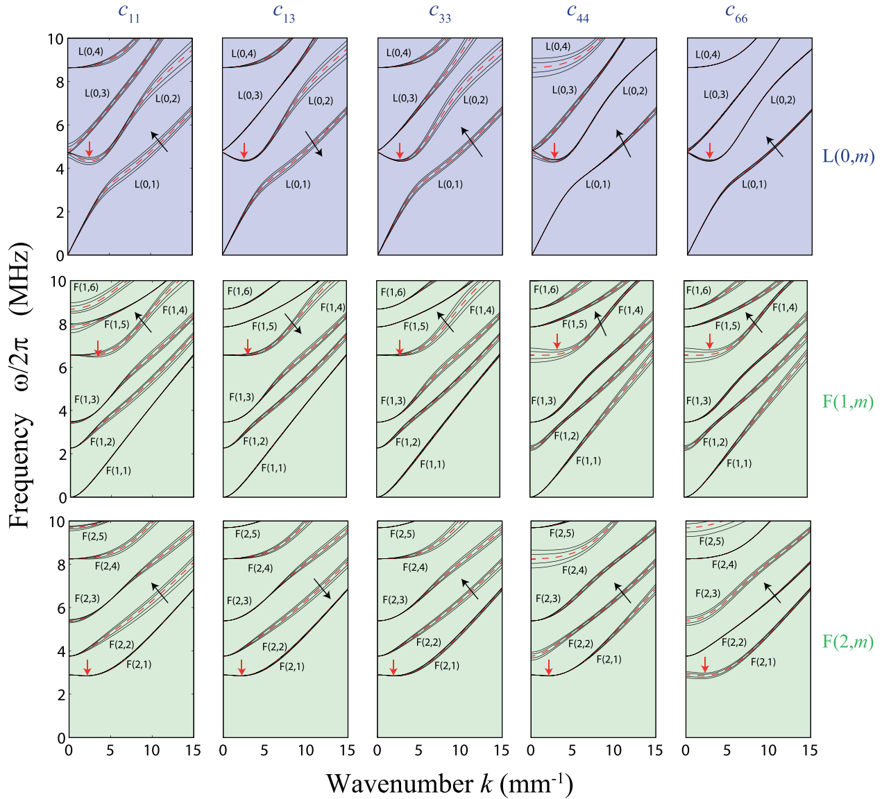
FIG. 4. (Color online) Influence of the elastic constants on the dispersion curves of a transversely isotropic cylinder. From top to bottom: for longitudinal modes and the first two flexural mode families. Vertical arrows depict the ZGV frequencies and tilted arrows show increasing c_{ij} .
