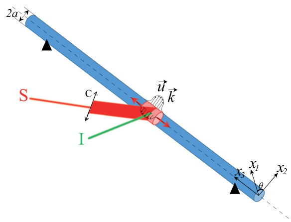
FIG. 1. (Color online) Source and probe geometry used to excite and to detect local resonances in a cylinder. S : laser source, I : interferometer, C : cylindrical lens.
