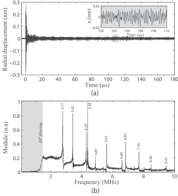
FIG. 3. (a) Radial displacement measured by the optical interferometer. Inset: zoom on a portion of the temporal displacement. (b) Frequency spectrum filtered by an analog high-pass filter ( f \leq 1.5 MHz).
