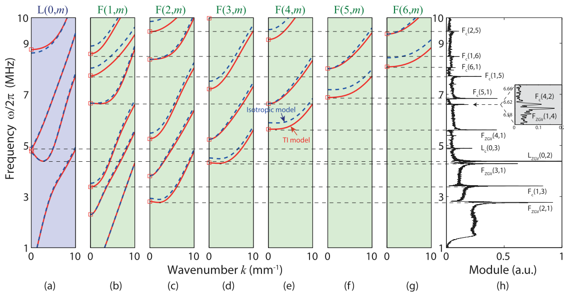
FIG. 6. (Color online) Comparison of isotropic model (dashed lines) with TI model (solid lines). (a) Longitudinal modes L(0, m) . (b)–(g) Flexural modes F(n, m) for n extends from 1 to 6. (h) Frequency spectrum recorded at epicenter. The subscript c denotes the cutoff frequencies. Inset: two resonance frequencies are observed corresponding to F(1, 4) -ZGV and F_c(4, 2) , respectively. The squares indicate the cutoff frequencies calculated with Eq. (6).
