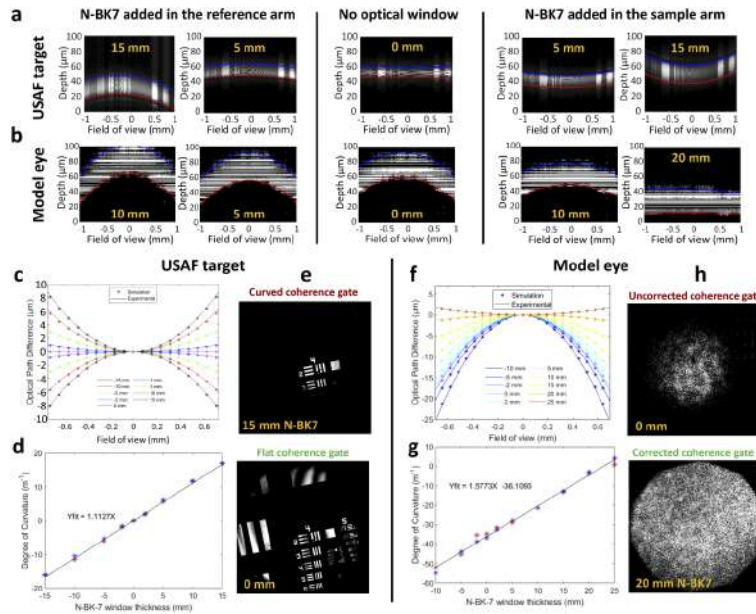
Fig. 3. a-b , Cross-sections after introducing N-BK7 optical windows with various thicknesses (in yellow) in the reference or sample arms when imaging the USAF target and the model eye. c,d,f,g , Measured and theoretical optical path differences as a function of the FOV for different optical window thicknesses, as well as their respective degree of curvature, for respectively the USAF target and the model eye. When the optical window was introduced in the reference arm, the N-BK7 optical window thickness was represented in negative value. e,h , The effect of the coherence gate geometry over the FF-OCT useful FOV.
