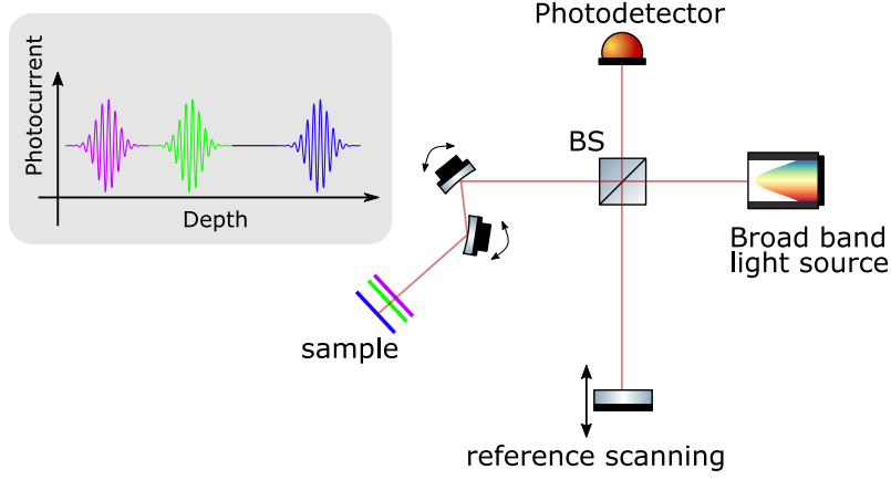
Fig. 1.2: TD-OCT simplified experimental setup. The sample is composed of 3 different reflective layers with the same reflectance.
