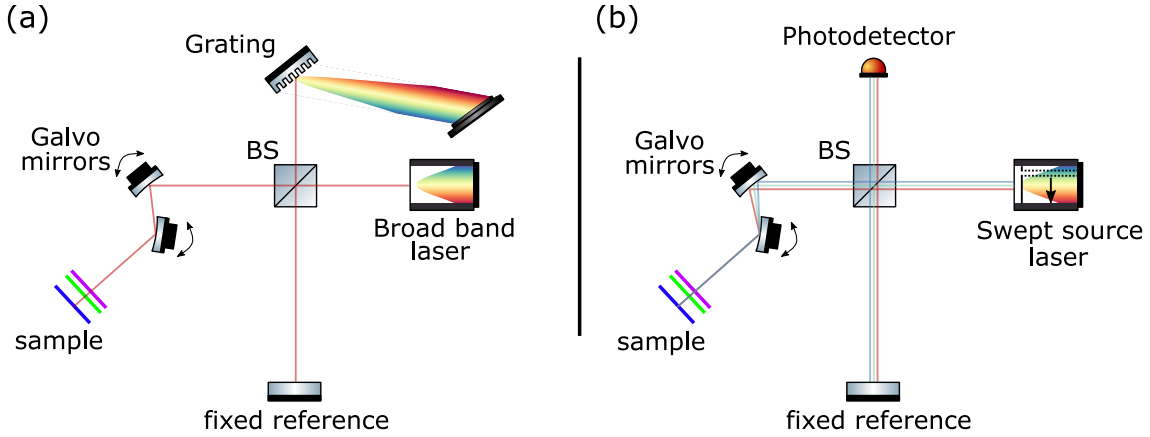
Fig. 1.3: FD-OCT simplified experimental setup. (a) SD-OCT setup: a broadband laser is used as illumination. The intensity is measured for each wavenumber \kappa and an inverse Fourier transform allows to obtain the axial distribution of reflectance R without mechanical scanning. (b) SS-OCT setup: a tunable laser is swept across the range of wavenumbers \Delta\kappa . The intensity is recorded for a collection of \kappa and the axial reflectance of the sample can again be obtained by an inverse Fourier transform.
