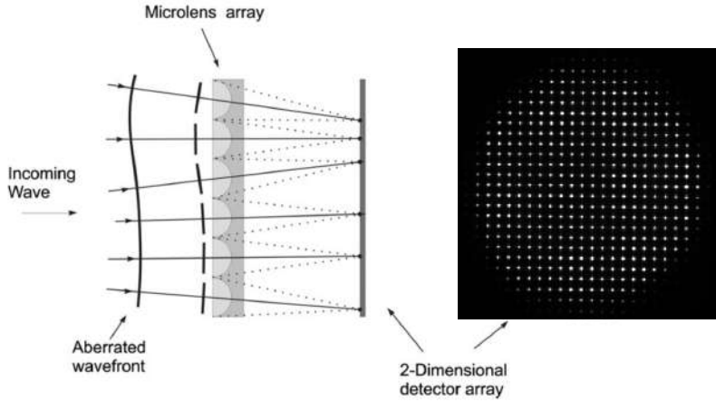
Fig. C.2: Shack-Hartmann WFS principle. A 2D array of lenslets with the same focal length is focusing the incoming beam onto a camera. Any phase aberration can be approximated by a set of local discrete tilts that are measured by the focal shift. By sampling the wavefront on the whole lenslet array it can be reconstructed with good accuracy.
