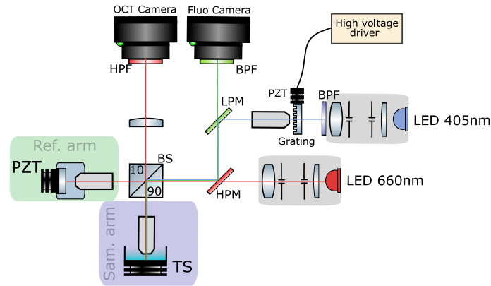
Fig. 5.2: HiLo combined with FFOCT setup. The ronchi rulling is 200 \text{ lp.mm}^{-1} and the microscope objective used to project the grid is a Olympus Plan N 10x 0.25NA.
