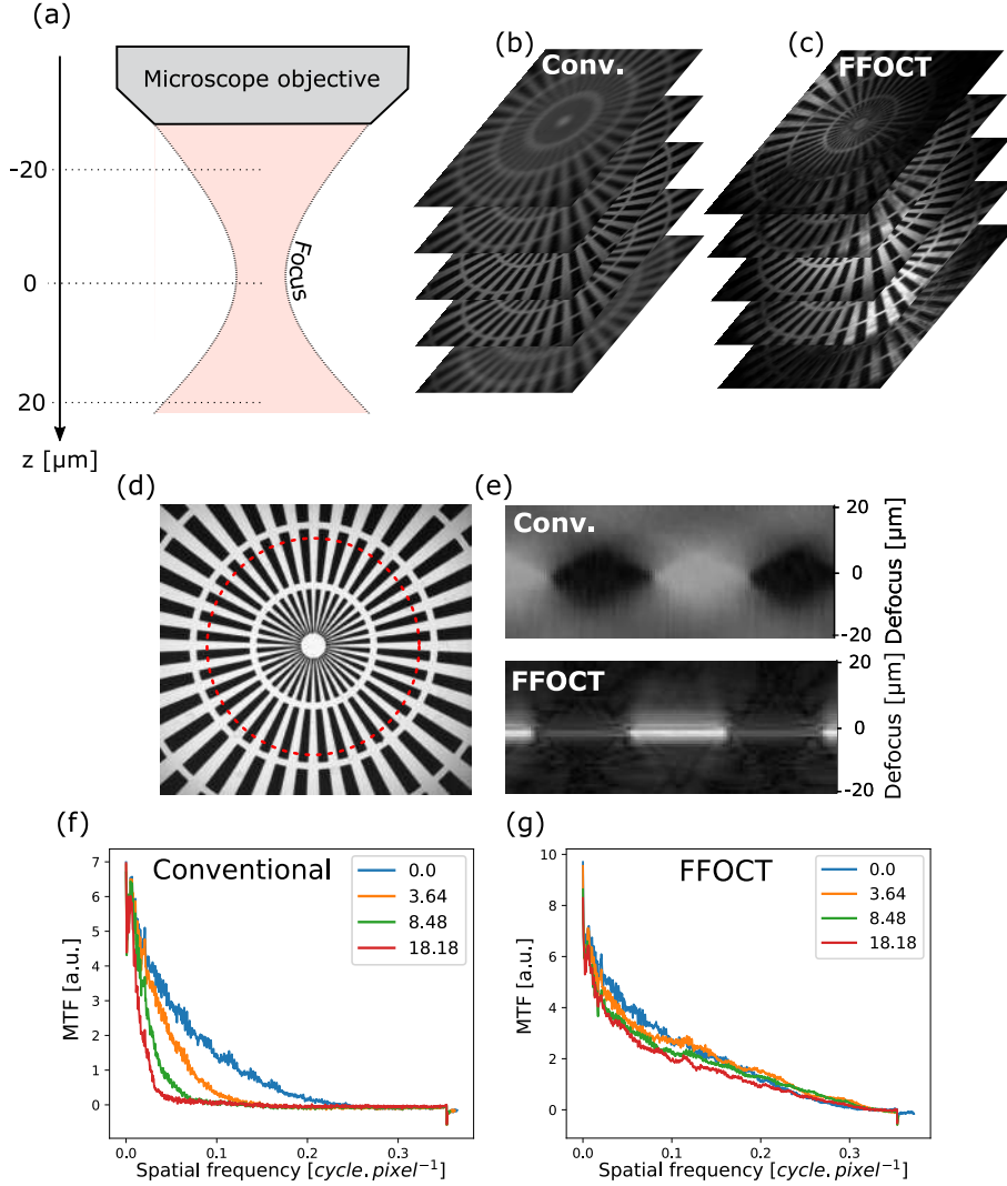
Fig. 4.8: Defocus experiment (a) A Siemens star target was imaged from -20 \mu\text{m} to 20 \mu\text{m} around the focal plane with 1 \mu\text{m} steps in (b) conventional images and (c) FFOCT. A radial reslice for constant spatial frequency (d) allow to see the difference in behavior for conventional systems compared to FFOCT (e). The MTF is approximated using a radial averaging of the Fourier transform magnitude for conventional images (f) and FFOCT (g). Each curve correspond to different amount of defocus adimensionned in NA/\lambda_c \mu\text{m} .
